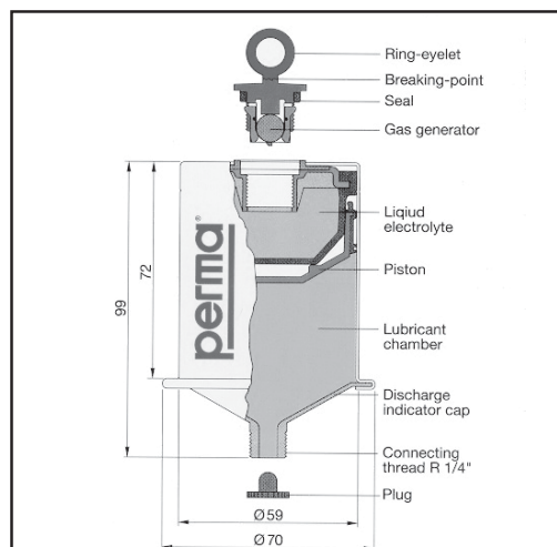
Automatic Lubricator Dimensions & Descriptions
