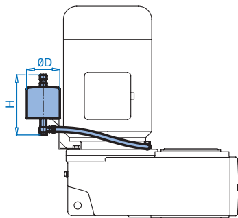
Oil Expansion Chamber Dimension Callouts
