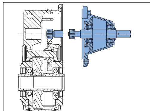
Solid Input Shaft
