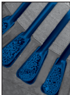
Insulation System
