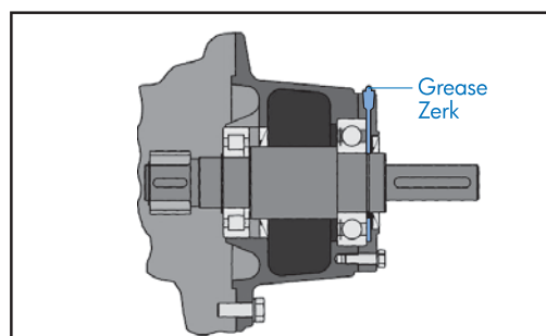
Re-Lubricating the bearing with the Grease Zerk
