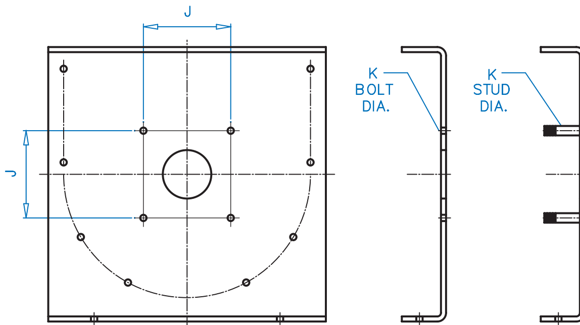
Screw Conveyor mounting dimensions from CEMA 300-13 excerpts
