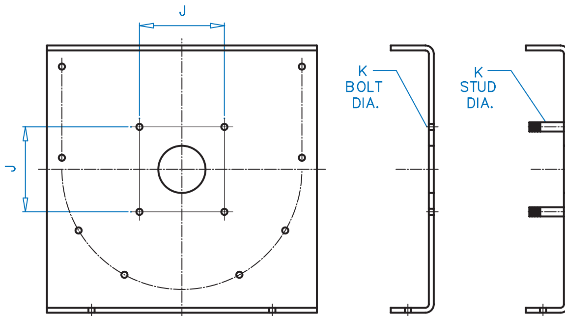
Screw Conveyor mounting dimensions from CEMA 300-13 excerpts
