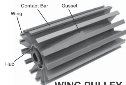
WING PULLEY
