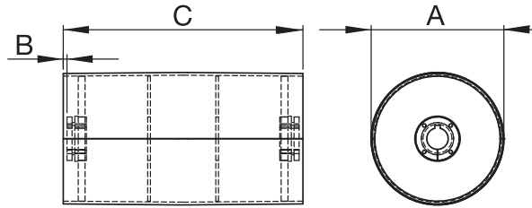
Standard Duty Drum — M-HE Bushed (Lagged)
