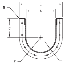
Angle Flange
