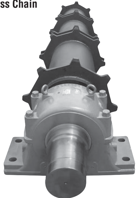
Sprocket Roller for Truck Dump in Sugar Mill Application
