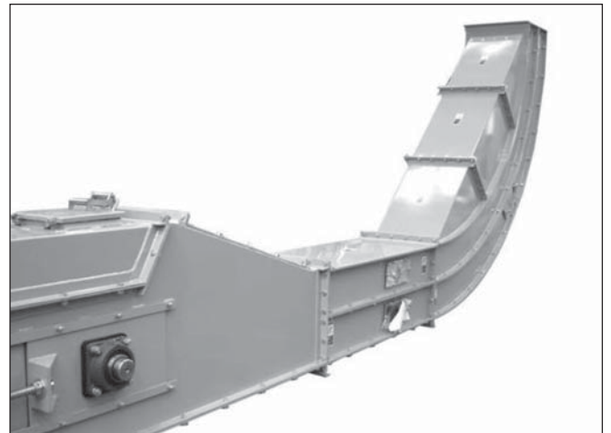
Tail Section and Stack Accommodate Lower Bend
