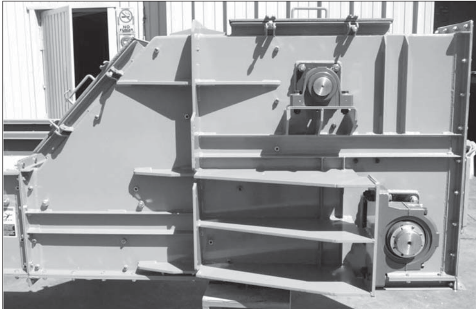
MMD Mill Duty Head with Thomas Slack Side Tension Idler Sprocket
