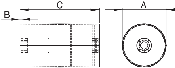
Standard Duty Drum Pulleys — M-HE Bushed
