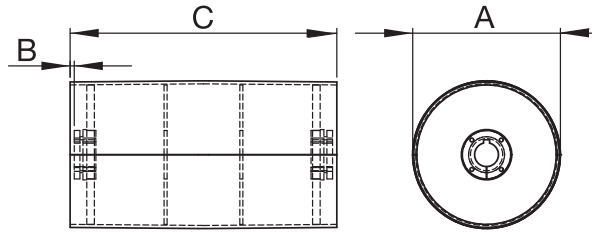
Mine Duty Drum Pulley — M-HE Bushed
