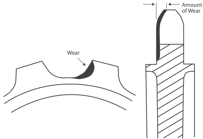
Sprocket Wear
