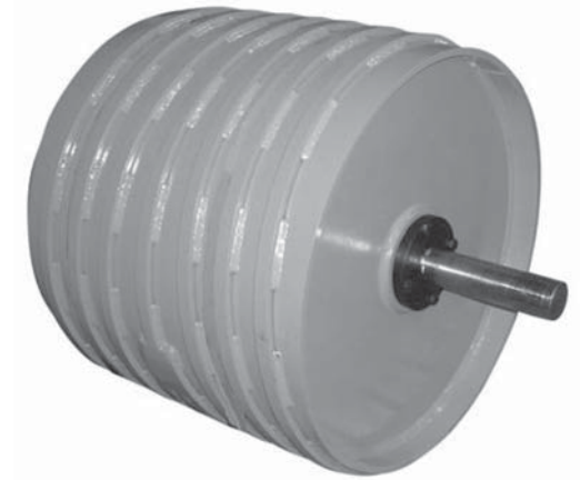
Spiral Drum Pulley with 1/2" x 1/2" Flight
