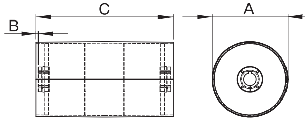
Standard Duty Drum Pulley
