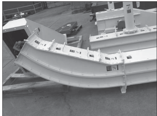
MMD Special L-Path Drag with Slack Accommodating Bend.
