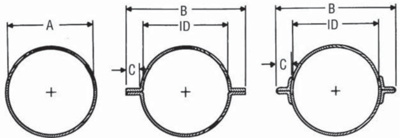
Tubular housing
