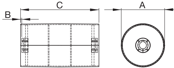
Mine Duty Drum Pulley (Lagged)
