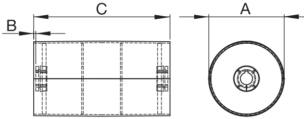
Standard Duty Drum (Lagged)
