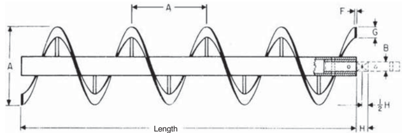
Ribbon Conveyor Screw
