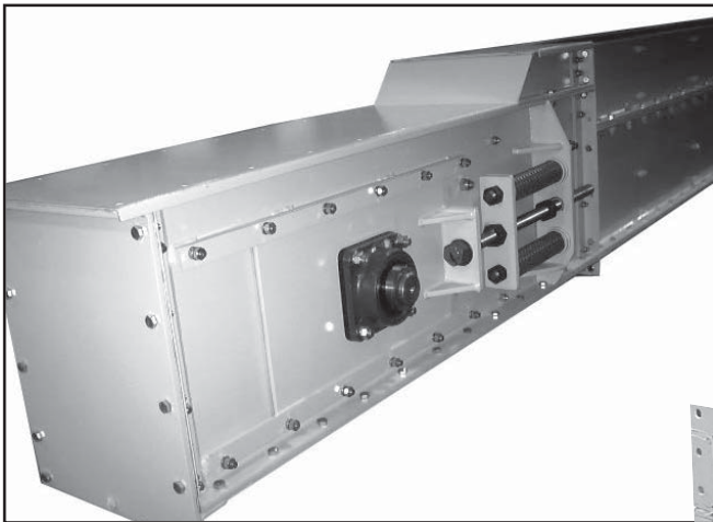
Feed Control Inlet and Spring Take-up on Thomas MMD Drag
