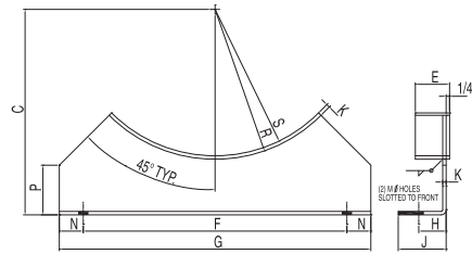
Saddle
