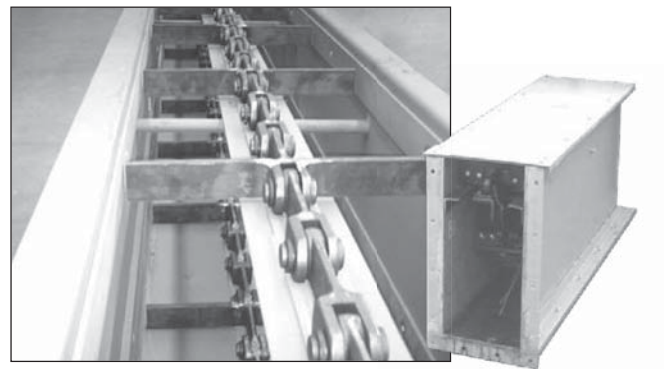
Center Support Rail Return System with AR steel Wear Strips for MMD Drag
