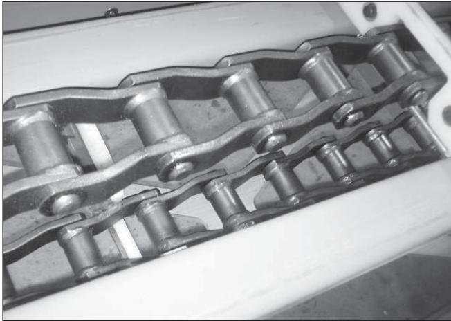
Weld Steel Chain and MFB Tail™
